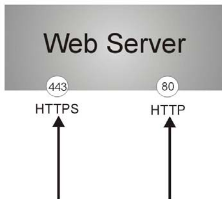
Figure 424 HTTP/HTTPS Implementation
