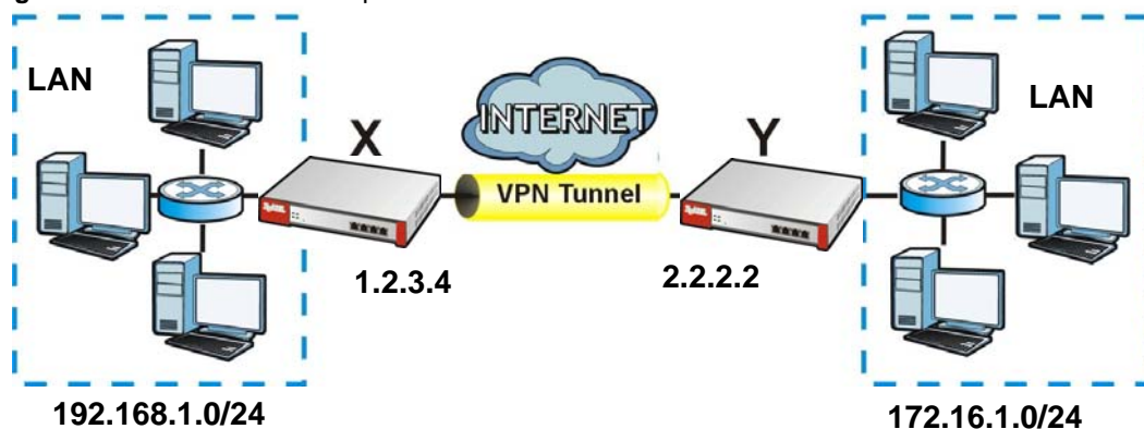
Figure 247 IPSec VPN Example
