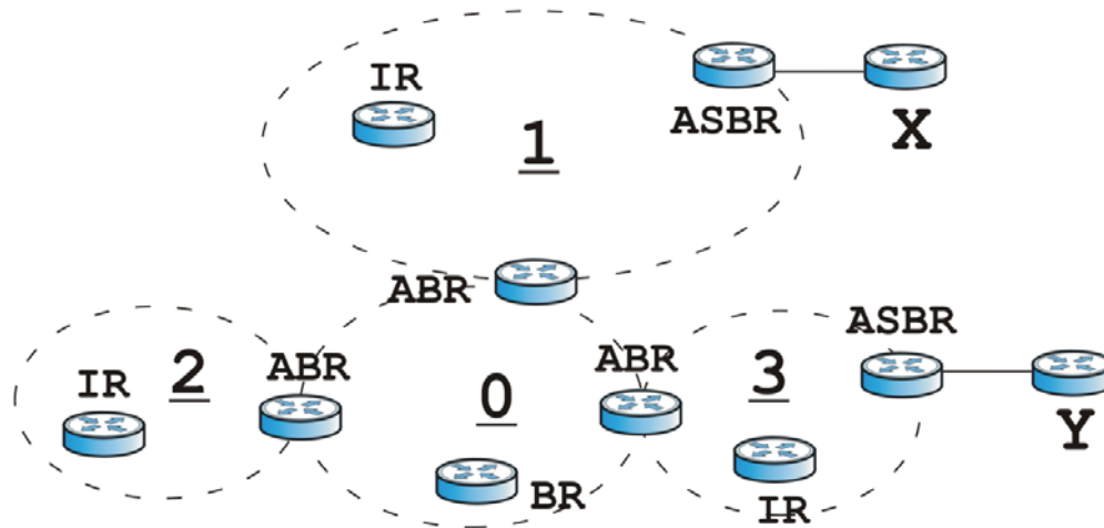
Figure 170 OSPF: Types of Routers
