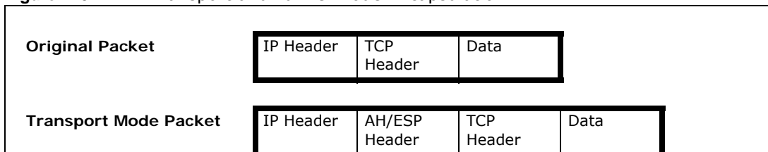
Figure 245 VPN: Transport and Tunnel Mode Encapsulation
