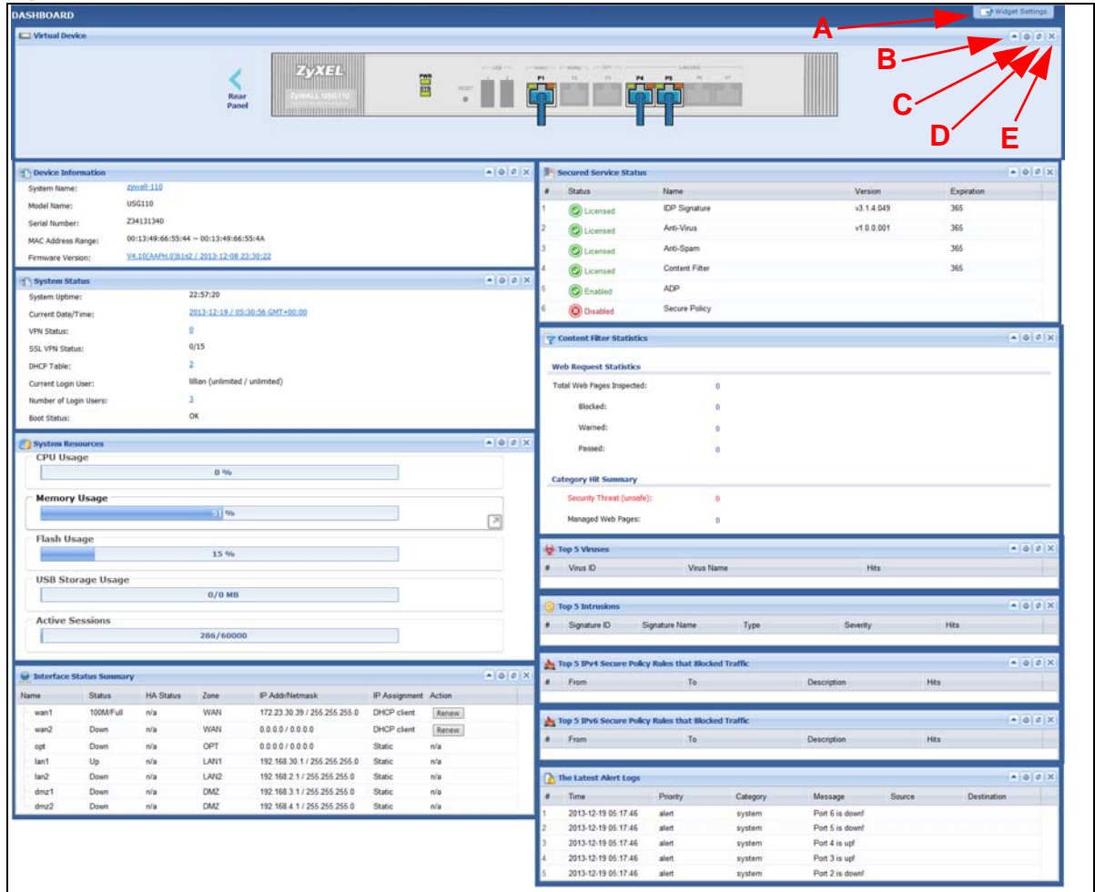
Figure 71 Dashboard
